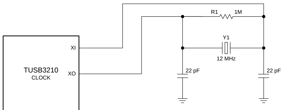
Figure 12. Crystal Implementation Diagram
