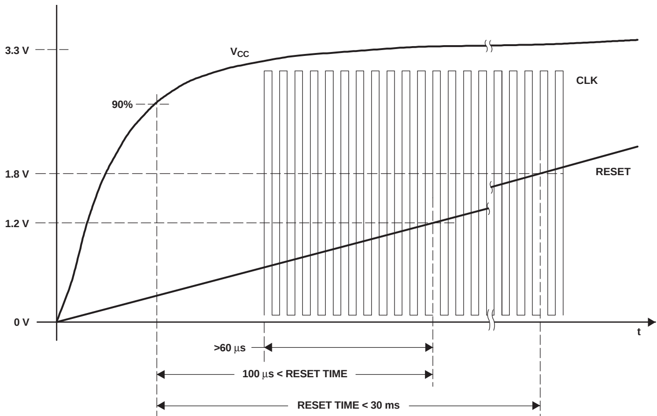
Figure 7. Reset Timing
