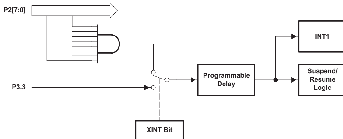
Figure 6. P2[7:0], P3.3 Input Port Interrupt Generation
