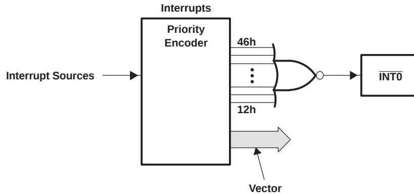
Figure 5. Internal Vector Interrupt ( \overline{\text{INT0}} )
