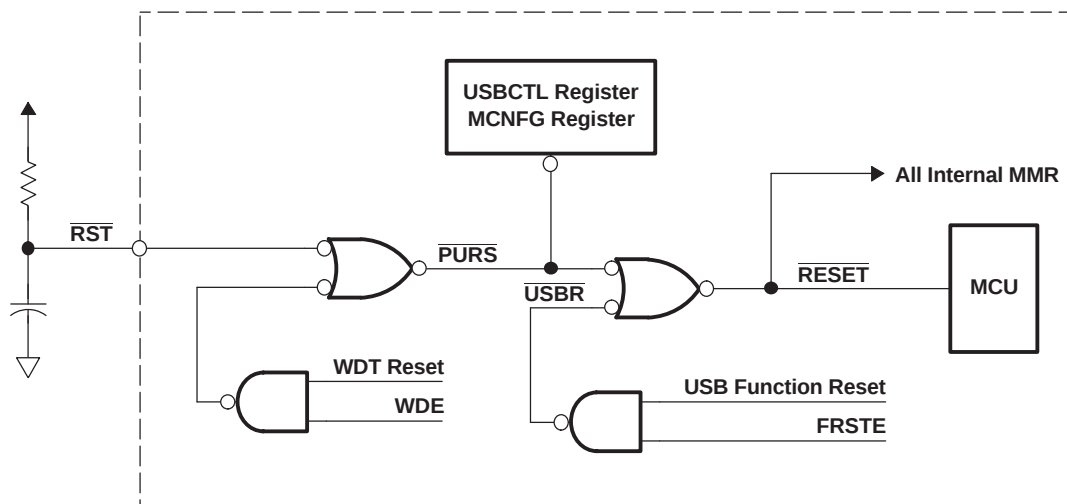
Figure 3. Reset Diagram
